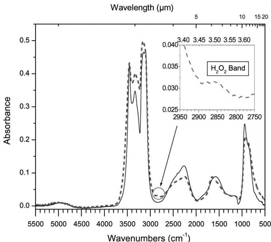
FIG. 2.—Infrared spectra of cubic crystalline water taken before irradiation (solid line) and after irradiation (dashed line) at 12 K. The inset enlarges the hydrogen peroxide absorption band centered at 2851\text{ cm}^{-1} ( 3.5\text{ }\mu\text{m} ). [See the electronic edition of the Journal for a color version of this figure.]
