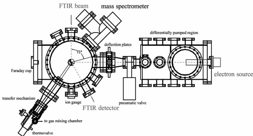
FIG. 1.—Top view of the experimental setup. [See the electronic edition of the Journal for a color version of this figure.]
