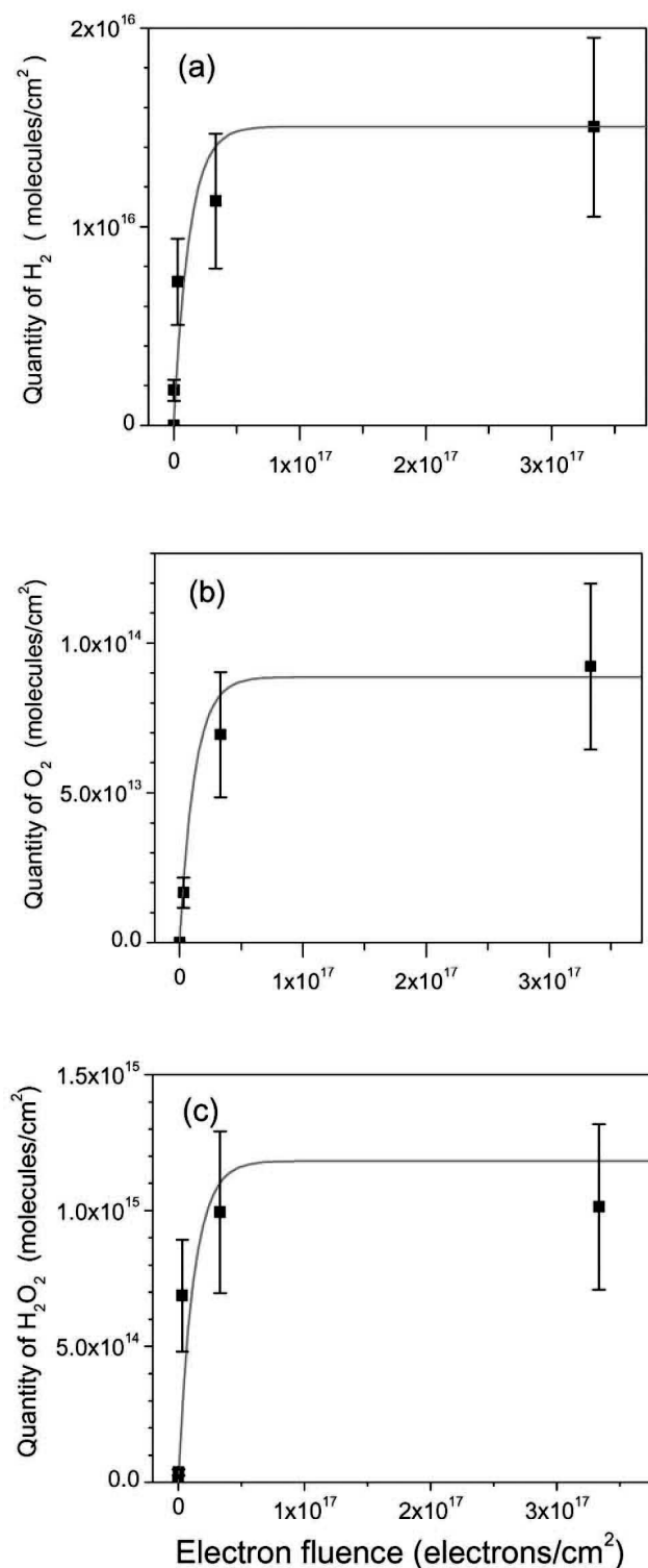
FIG. 7.—Quantification of the numbers of (a) molecular hydrogen (H 2 ), (b) molecular oxygen (O 2 ), and (c) hydrogen peroxide (H 2 O 2 ) as a function of the irradiation electron fluence. [See the electronic edition of the Journal for a color version of this figure.]
