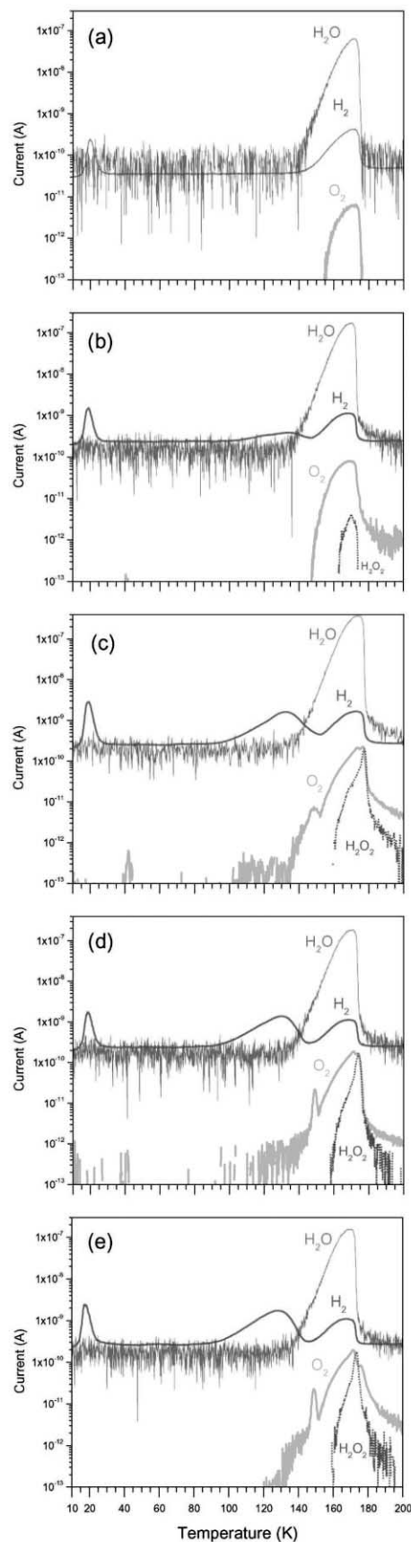
FIG. 6.—Temporal evolution of the ion currents of molecular hydrogen ( \text{H}_2 ), molecular oxygen ( \text{O}_2 ), hydrogen peroxide ( \text{H}_2\text{O}_2 ), and water ( \text{H}_2\text{O} ) during the warm-up phase experiment for (a) 0, (b) 10, (c) 100, (d) 1000, and (e) 10,000 nA. [See the electronic edition of the Journal for a color version of this figure.]
