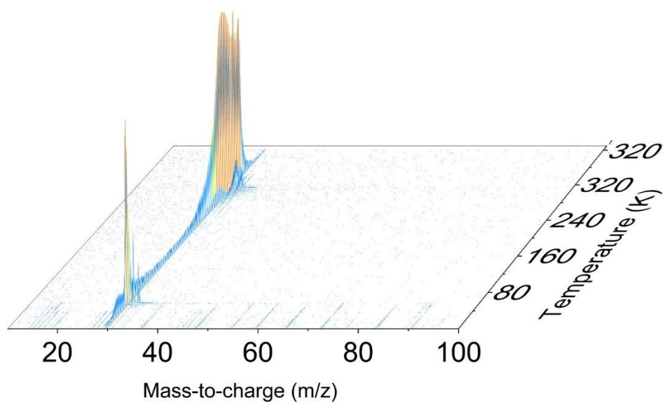
Fig. S7. PI-ReTOF mass spectrum measured at a photon energy of 10.49 eV during the TPD phase of non-irradiated methane ( \text{CH}_4 ) and nitrogen monoxide ( \text{NO} ) ice mixture i.e. blank experiment.
