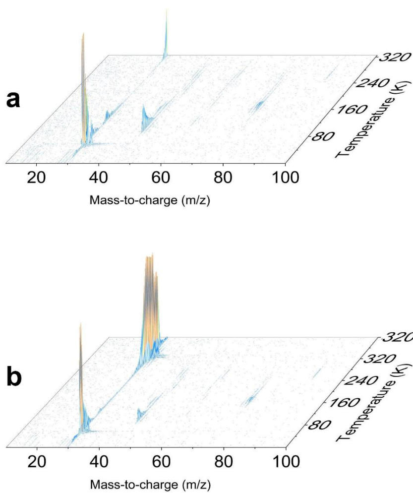
Fig. S6. PI-ReTOF mass spectra measured at photon energies of (a) 9.95 eV and (b) 9.92 eV during the TPD phase of irradiated methane ( \text{CH}_4 ) and nitrogen monoxide ( \text{NO} ) ice mixture.
